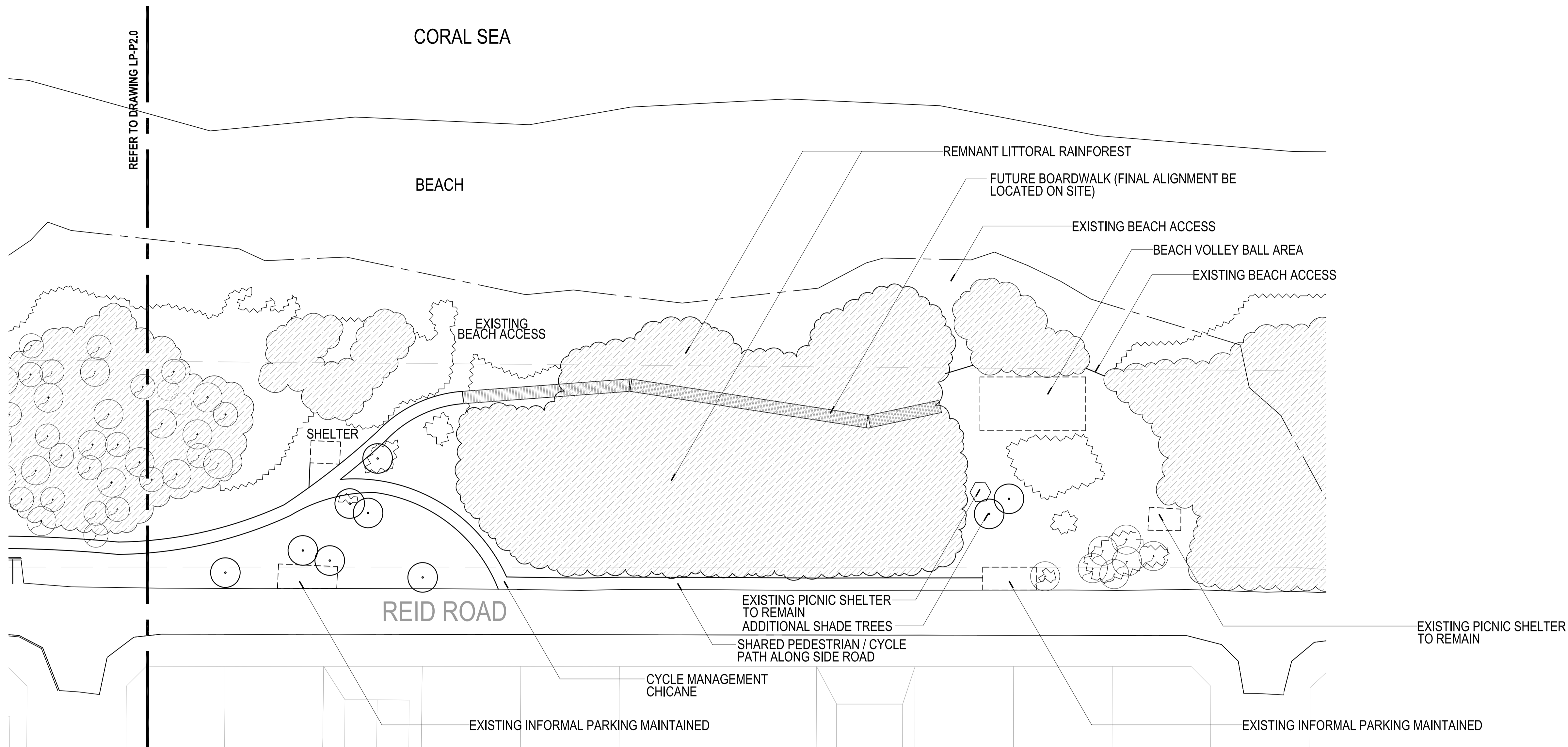
01 SITE PLAN SCALE 1:500 @ A1 / 1:1000 @ A3
